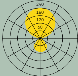
oto 10/46 151lm/W@4000K
