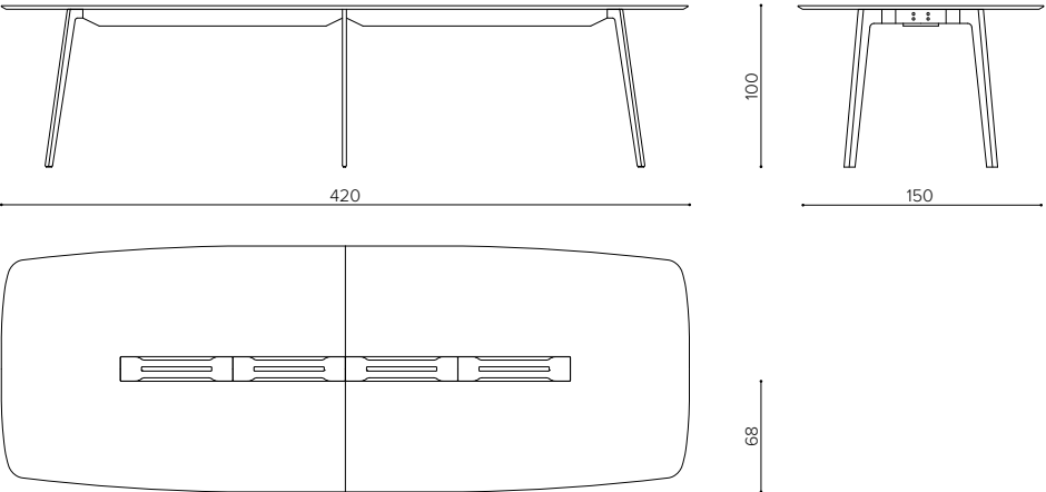
WI 420H high table 420x150x100 cm tavolo alto 420x150x100 cm tavolo haute 420x150x100 cm
