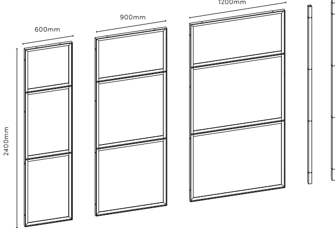
H2400MM - Perspective
