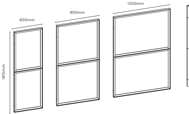
H1800MM - Perspective
