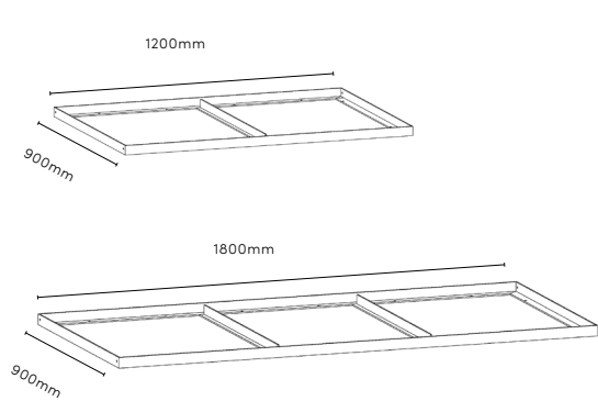
D900MM - Perspective
