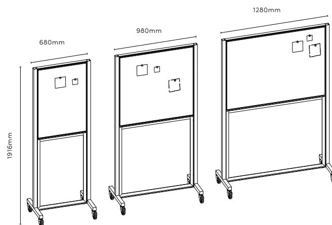
H1800MM - Perspective
