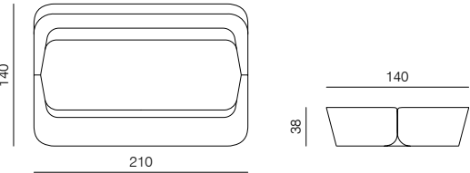
3SEATER SOFA BED OPENED dimensions 210 × 140 × 38 cm
