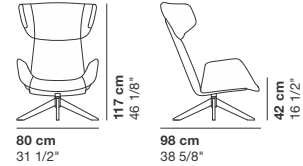
cod. 9055 / wood_swivel lounge chair
