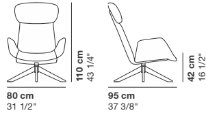
cod. 9054 / wood_swivel lounge chair
