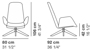
cod. 9053 / wood_swivel lounge chair
