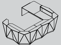
ALP27L 3815 / 3135 / 1100 150 1/4" / 123 3/8" / 43 1/4" ALP27P 3815 / 3135 / 1100 150 1/4" / 123 3/8" / 43 1/4"
