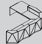
ALP24L 3967 / 3135 / 1100 156 1/8" / 123 3/8" / 43 1/4" ALP24P 3967 / 3135 / 1100 156 1/8" / 123 3/8" / 43 1/4"
