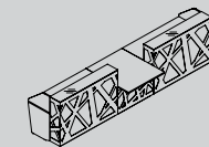
LZG52 4200 / 1180 / 1146 165 1/2" / 46 1/2" / 45 1/8" LZG53 4800 / 1180 / 1146 189 1/8" / 46 1/2" / 45 1/8" LZG54 5400 / 1180 / 1146 212 3/4" / 46 1/2" / 45 1/8"
