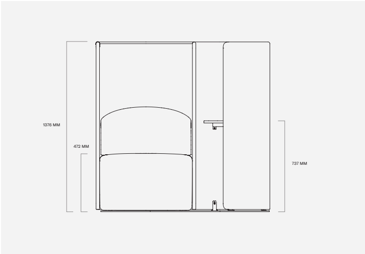
TULIPAN front view / open
