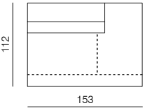
1SEATER EXTENDED 153 (L/R) dimensions 153 × 112 × 70 cm
