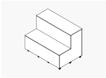
Module 9 Large with castors W: 1350 x D: 900 x H: 940 mm
