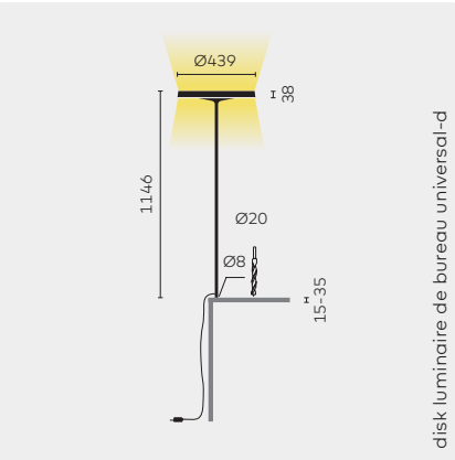
disk suspension
